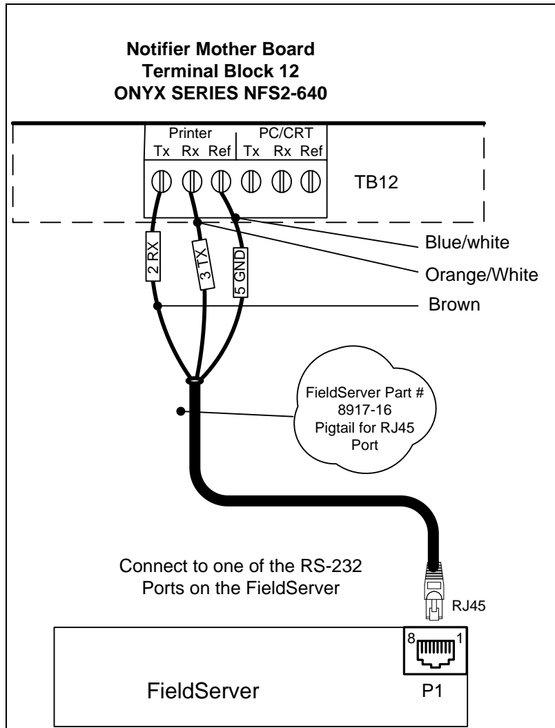
Figure 2: Diagram showing connection to the NFS2-640 Panel Printer Port
